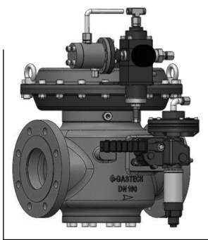
Gas Pressure Regulator with Slum Shut Valve + Monitor F65-150M/S Serie
