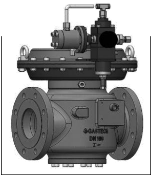
Gas Pressure Regulator F65-150
