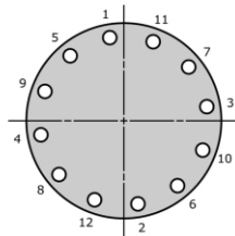
Circular 12-Bolt
