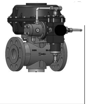
Gas Pressure Regulator F25-50
