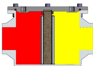
Threaded Connection Gas Filter
